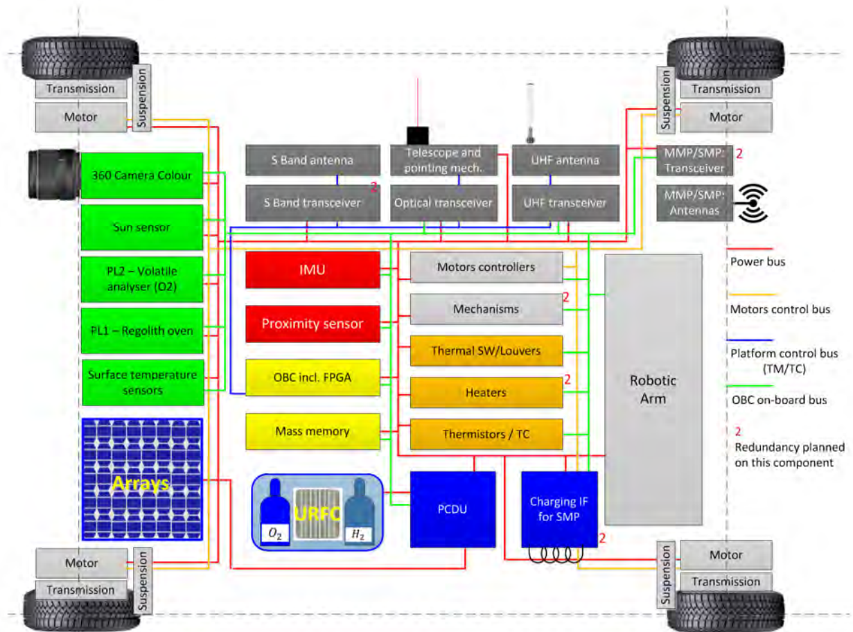
Figure 4.2: MMP architecture and subsystems
